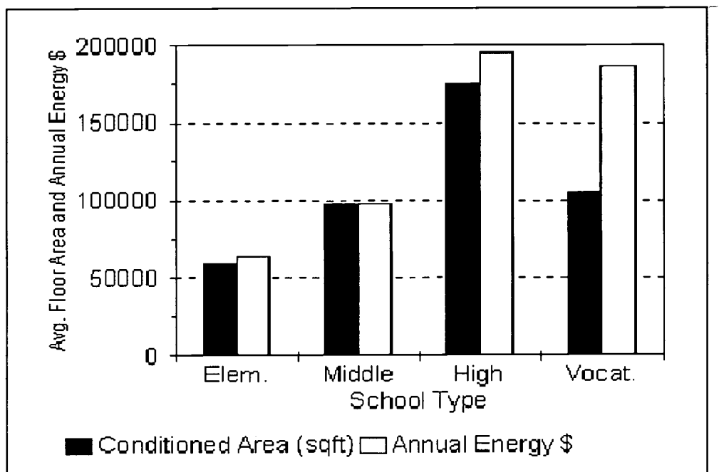
Figure 2. Variation of conditioned floor area and annual energy cost by school type.
